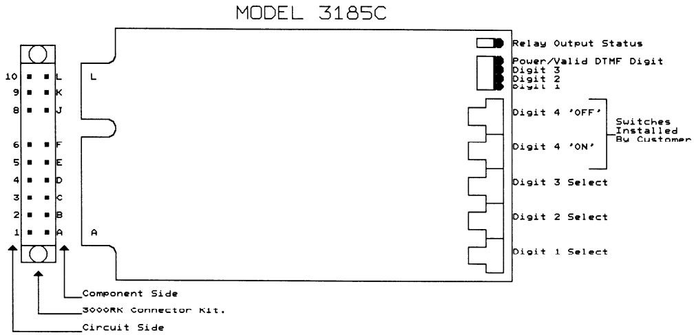
FIGURE 1 Edge Connector, Switch, and Indicator Locations
