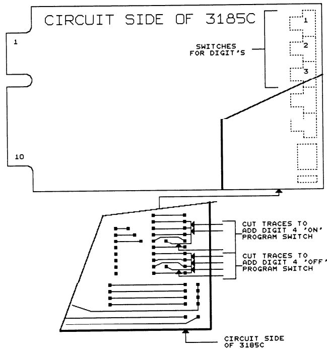
FIGURE 4 MODIFYING BOARD FOR PROGRAM SWITCHES
